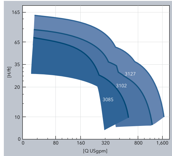
Performance, 60 Hz
